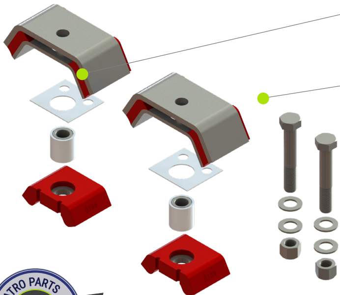
KT59-62004-HT (xxx) Engine Mount Kit w/Hardware, Rear (High Temp)
